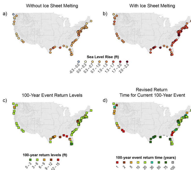
Projected Sea Level Rise and Flooding by 2050
